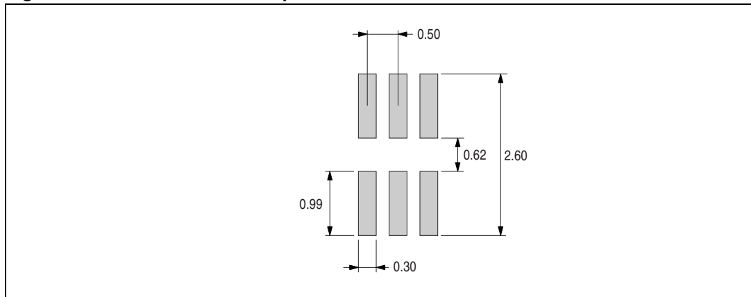
Figure 17. Recommended footprint
