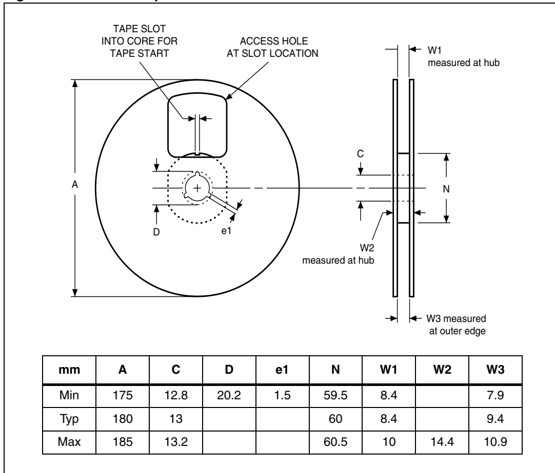
Figure 18. Reel description
