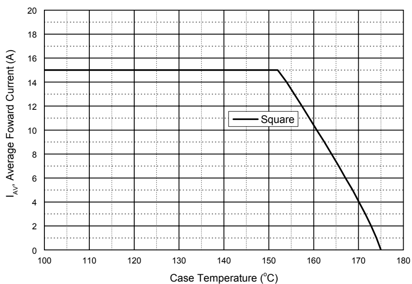
Figure 7. Average Forward Current vs. Case Temperature (Square, Each Diode)
