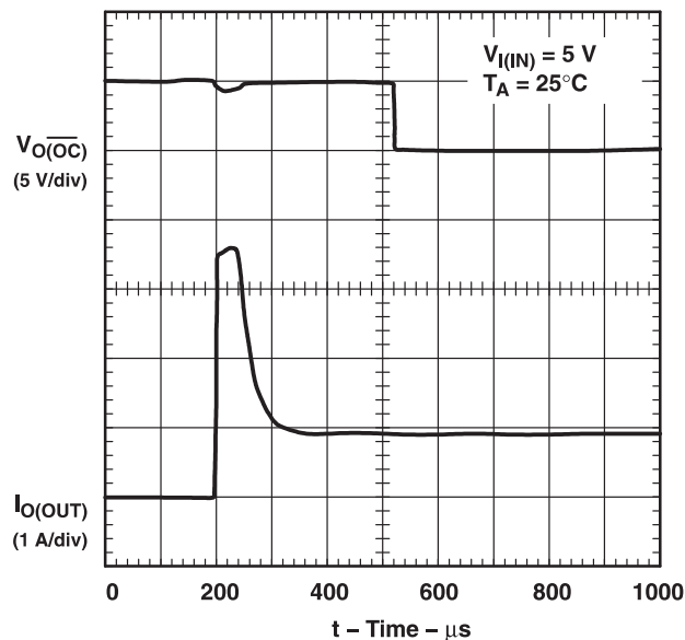
Figure 11. 1-Ω Load Connected to Enabled Device
