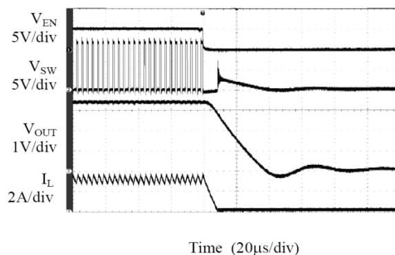
Fig. 13: Enable turn off CC mode, I_{OUT}=3A
