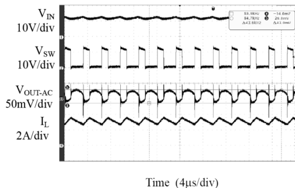
Fig. 10: Output voltage ripple, I_{OUT}=3A
