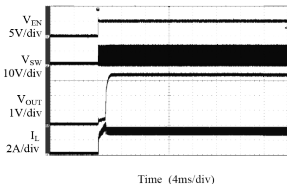
Fig. 12: Enable turn on CC mode, I_{OUT}=3A
