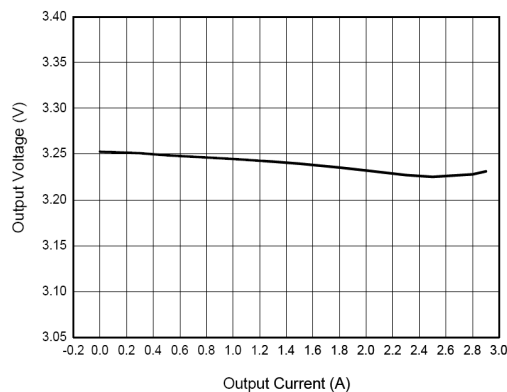
Fig. 9: Output voltage versus output current
