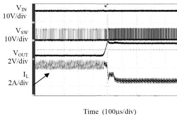
Fig. 15: Short-circuit recovery, I_{OUT}=3A
