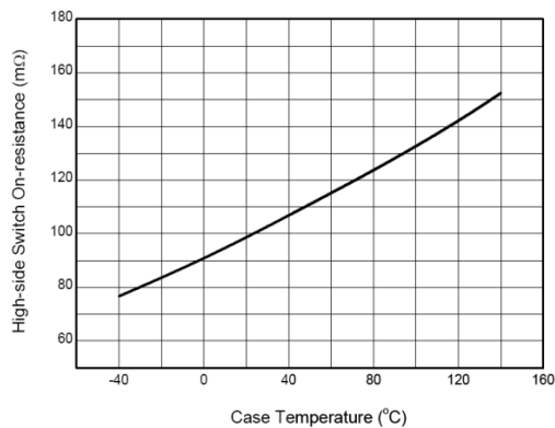
Fig. 5: R_{DS(on)} versus case temperature
