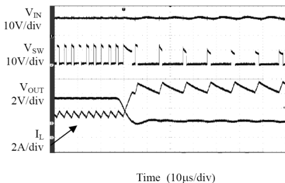
Fig. 14: Short-circuit protection, I_{OUT}=3A
