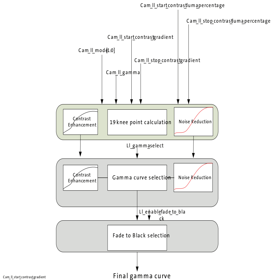
Figure 23: Gamma Interaction
