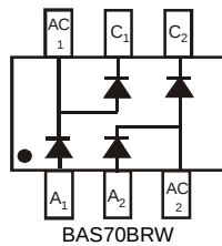
BAS70BRW
