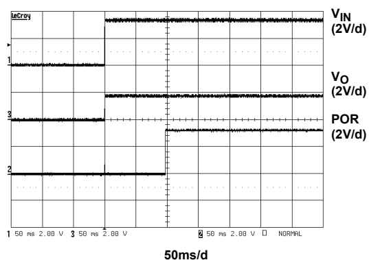
FIGURE 8. START-UP 2
