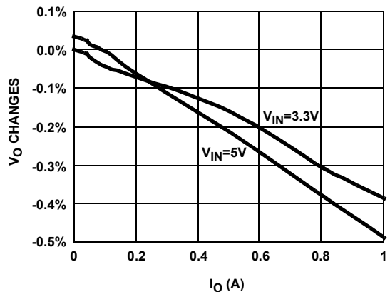
FIGURE 4. LOAD REGULATIONS
