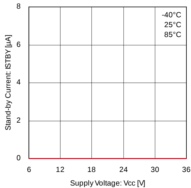
Fig.4 Stand-by current
