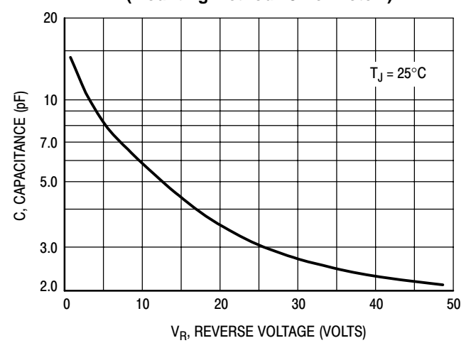
Figure 10. Typical Capacitance
