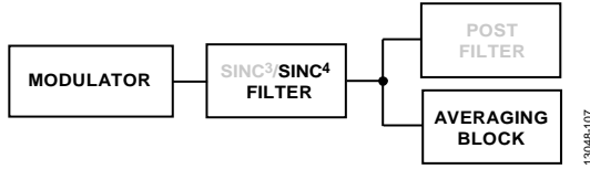
Figure 97. Fast Settling Mode, Sinc 4 + Sinc 1 Filter
