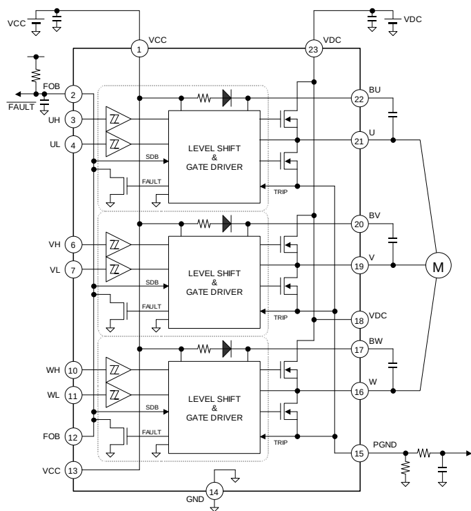
Figure 2. Block Diagram
