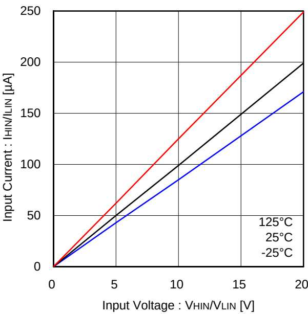
Figure 18. Input Bias Current (UH,UL,VH,VL,WH,WL)
