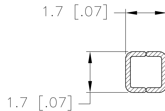
SECTION C-C
