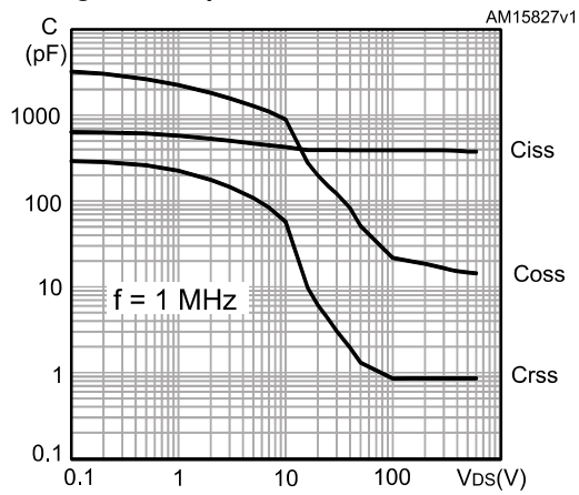
Figure 8: Capacitance variations
