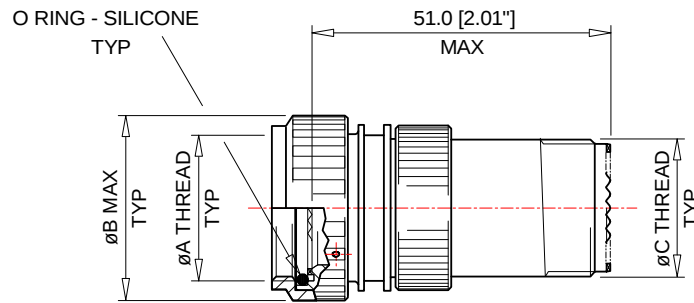
STRAIGHT ADAPTOR -00
