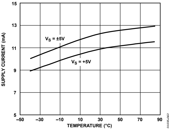
Figure 54. Supply Current vs. Temperature
