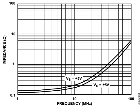
Figure 12. Closed-Loop Single-Ended Z_{OUT} vs. Frequency; G = +1 (See Figure 56)
