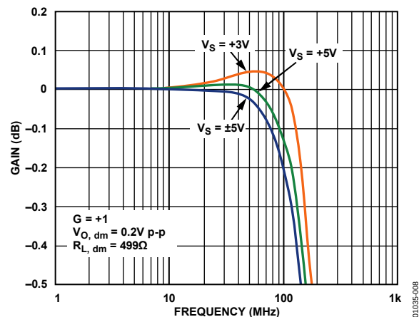
Figure 7. 0.1 dB Flatness vs. Frequency; C_F = 0.5 pF (See Figure 56)
