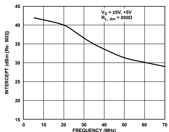
Figure 34. Third-Order Intercept vs. Frequency, G = +1
