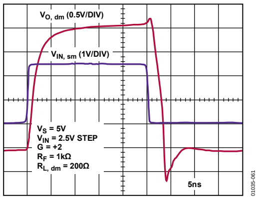
Figure 53. Overdrive Recovery
