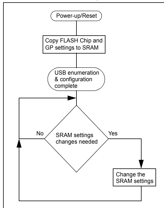
FIGURE 1-1: CHIP SETTINGS RUNTIME MANAGEMENT
