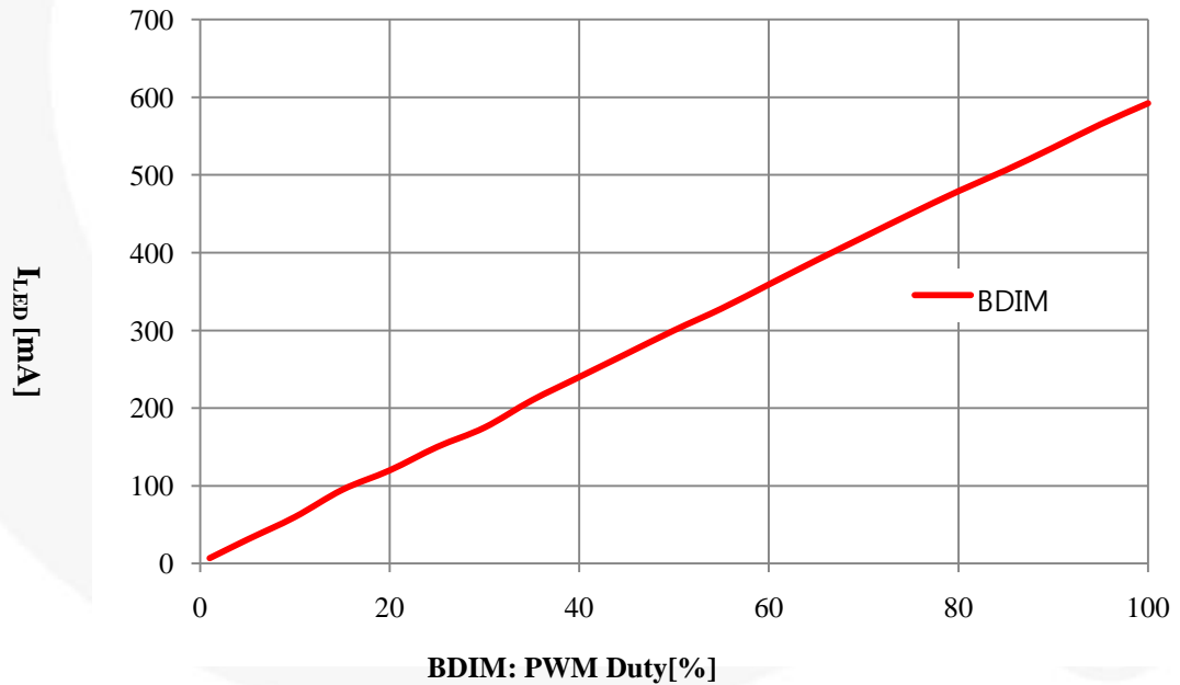
Figure 70. PWM Characteristics
