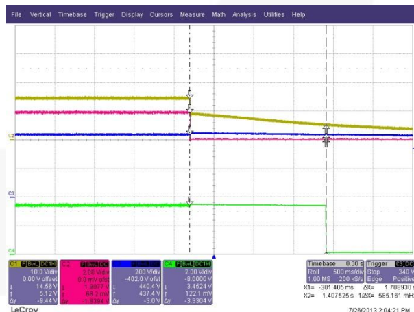
Figure 32. PS-OFF, [500 ms/div]
