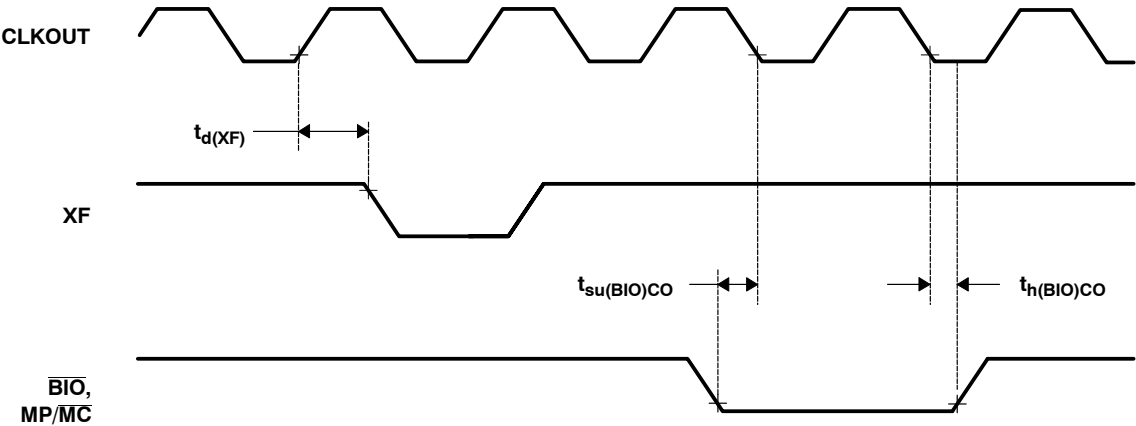
Figure 35. XF and \overline{\text{BIO}} Timing
