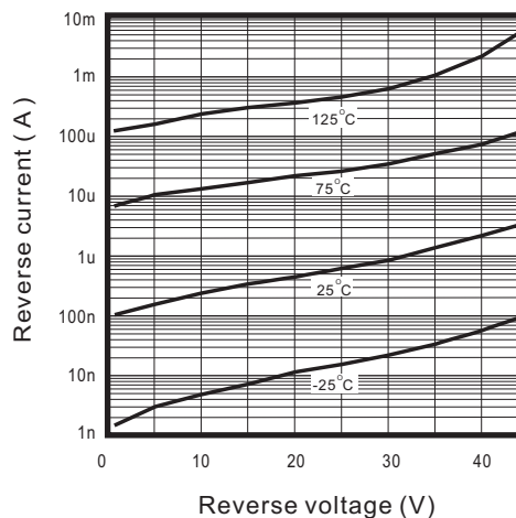
Fig. 2 - Reverse characteristics
