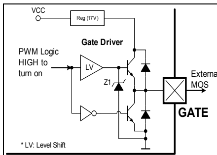
Figure 14 Gate Driver
