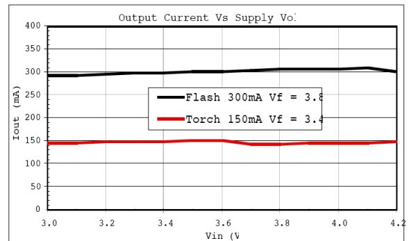
Fig. 13: Output Current vs Supply Voltage D1=AOT3228HPW0303B LED, R_{SENSE}=0.3\Omega R_{SET}=140k\Omega , C_{IN}=2.2\mu F , C_{FC}=0.47\mu F , C_{OUT}=1\mu F
