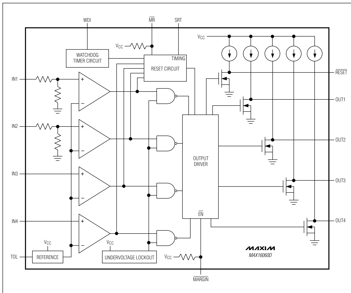
Figure 1. MAX16060D Functional Diagram
