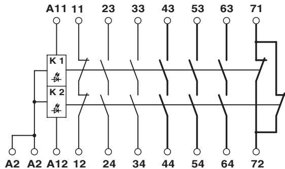
Figure 1 Block diagram
