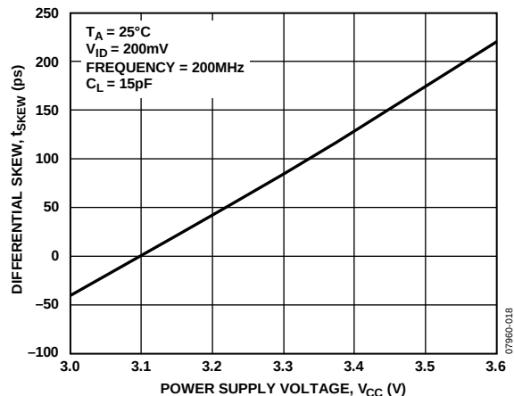
Figure 15. Differential Skew vs. Power Supply Voltage
