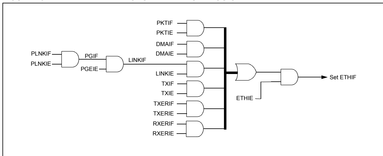
FIGURE 19-7: ETHERNET MODULE INTERRUPT LOGIC
