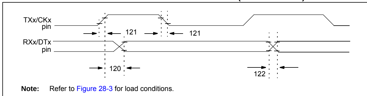
FIGURE 28-19: EUSARTx SYNCHRONOUS TRANSMISSION (MASTER/SLAVE) TIMING
