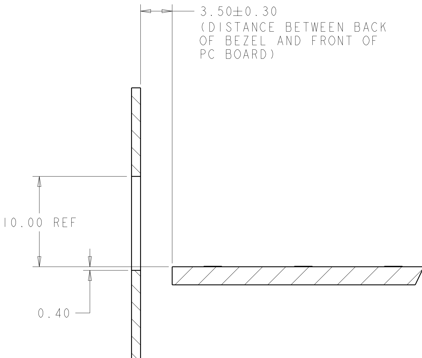
SECTION X-X
