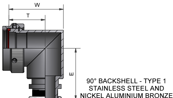
90° BACKSHELL - TYPE 1
