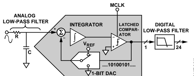
Figure 17. First-Order \Sigma - \Delta ADC
