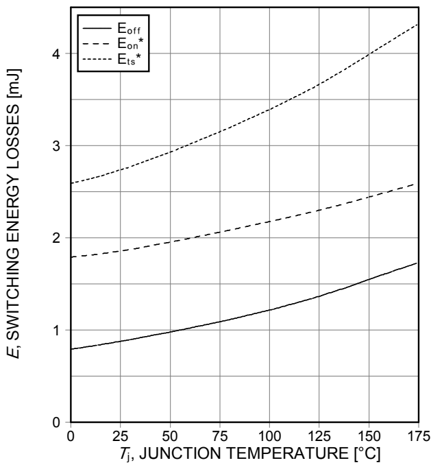
Figure 15. Typical switching energy losses as a function of junction temperature (ind. load, V_{CE}=600\text{V} , V_{GE}=15/0\text{V} , I_c=25\text{A} , R_G=23\Omega , test circuit in Fig. E)
