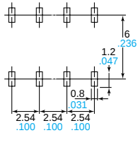
Recommended mounting pad (Top view)
