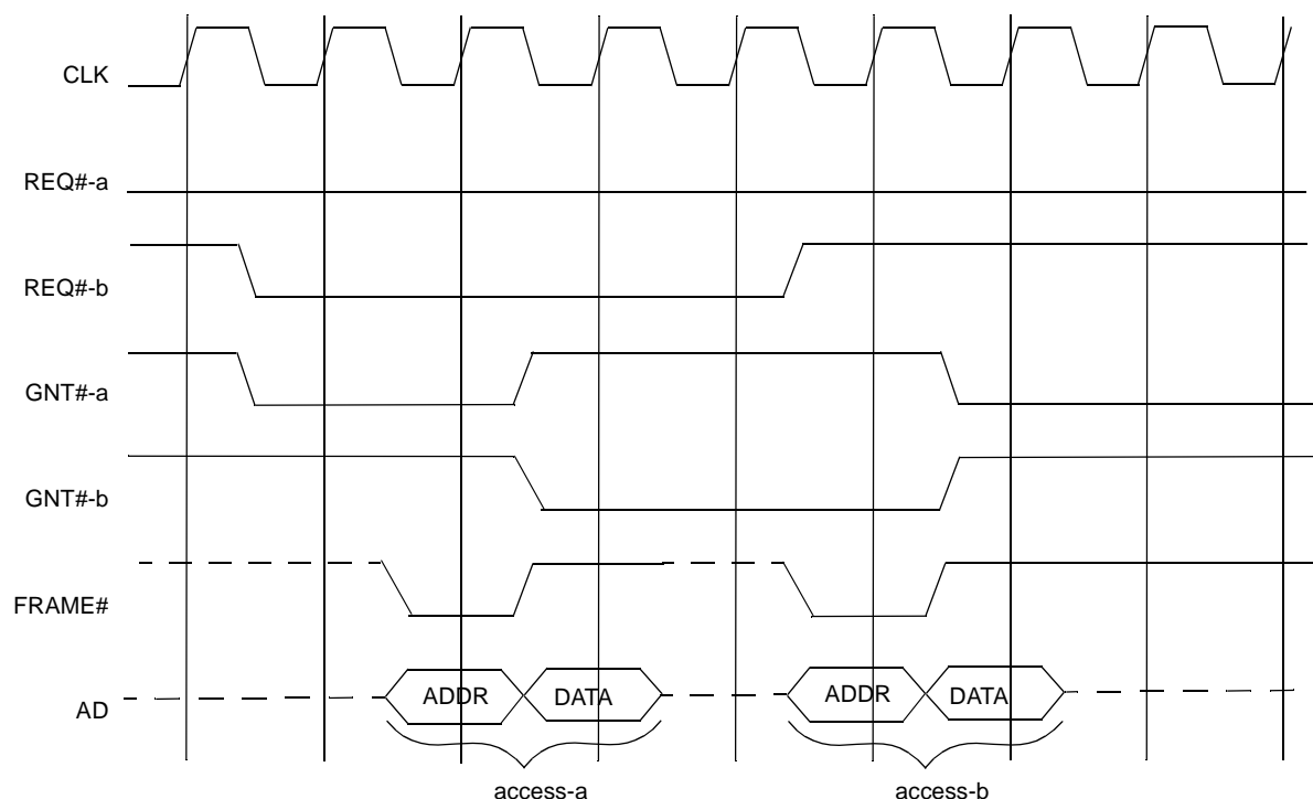
Figure 4-20. Basic Arbitration
