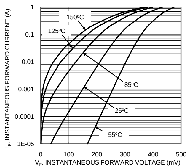
Figure 4. Typical Forward Characteristics
