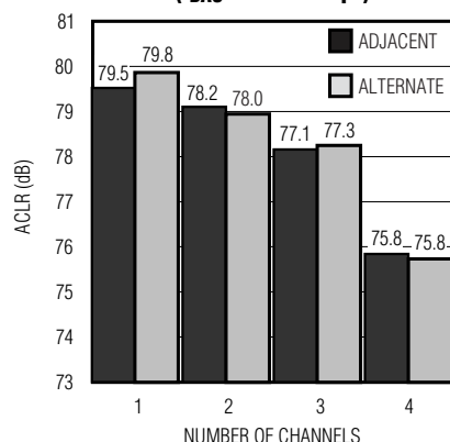
WCDMA BASEBAND ACLR ( f_{DAC} = 245.76Mps )
