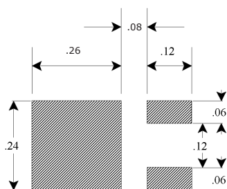
TO-252-2
