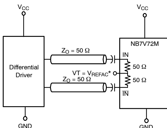
Figure 16. Capacitor-Coupled Differential Interface
