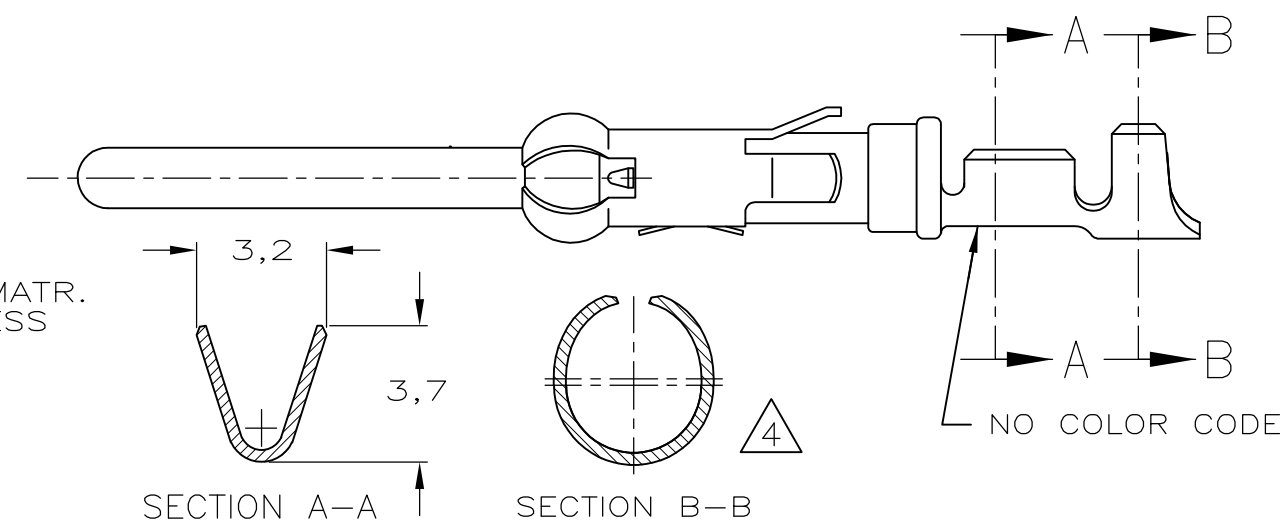
LOOSE PIECE
