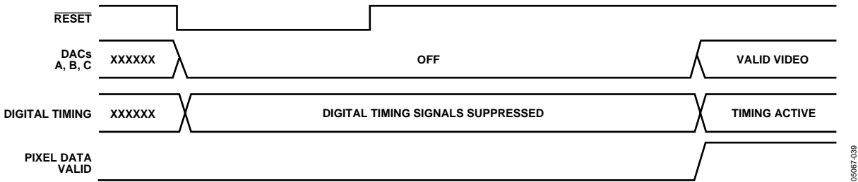
Figure 63. RESET Timing Sequence
