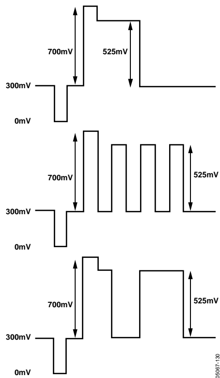
Figure 130. SD RGB Output Levels—RGB Sync Enabled
