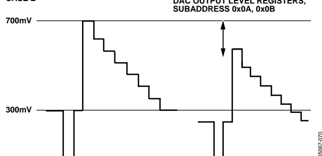
Figure 70. Programmable DAC Gain—Positive and Negative Gain
