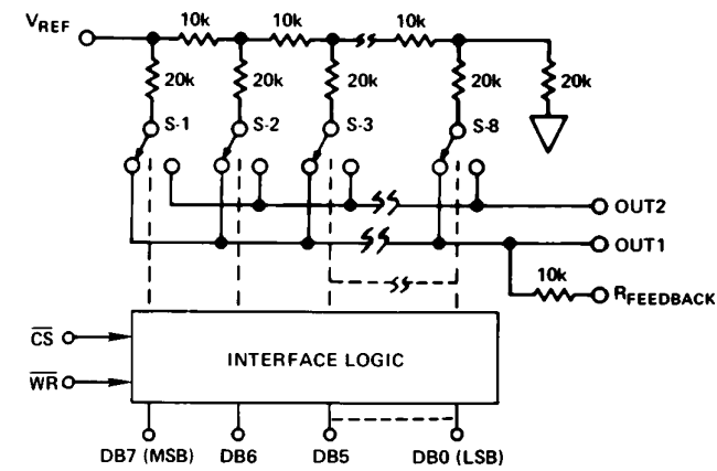
Figure 1. Functional Diagram
