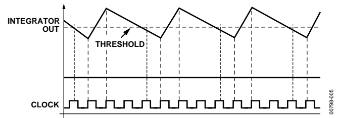
Figure 5. Integrator Output for I_{IN} = 250 \mu A
