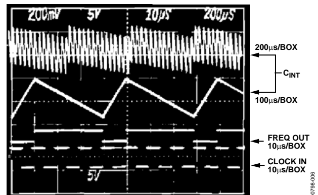
Figure 6. Integrator Output for I_{IN} Slightly Greater than 250 \mu A
