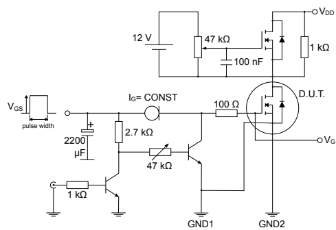
Figure 15. Gate charge test circuit
