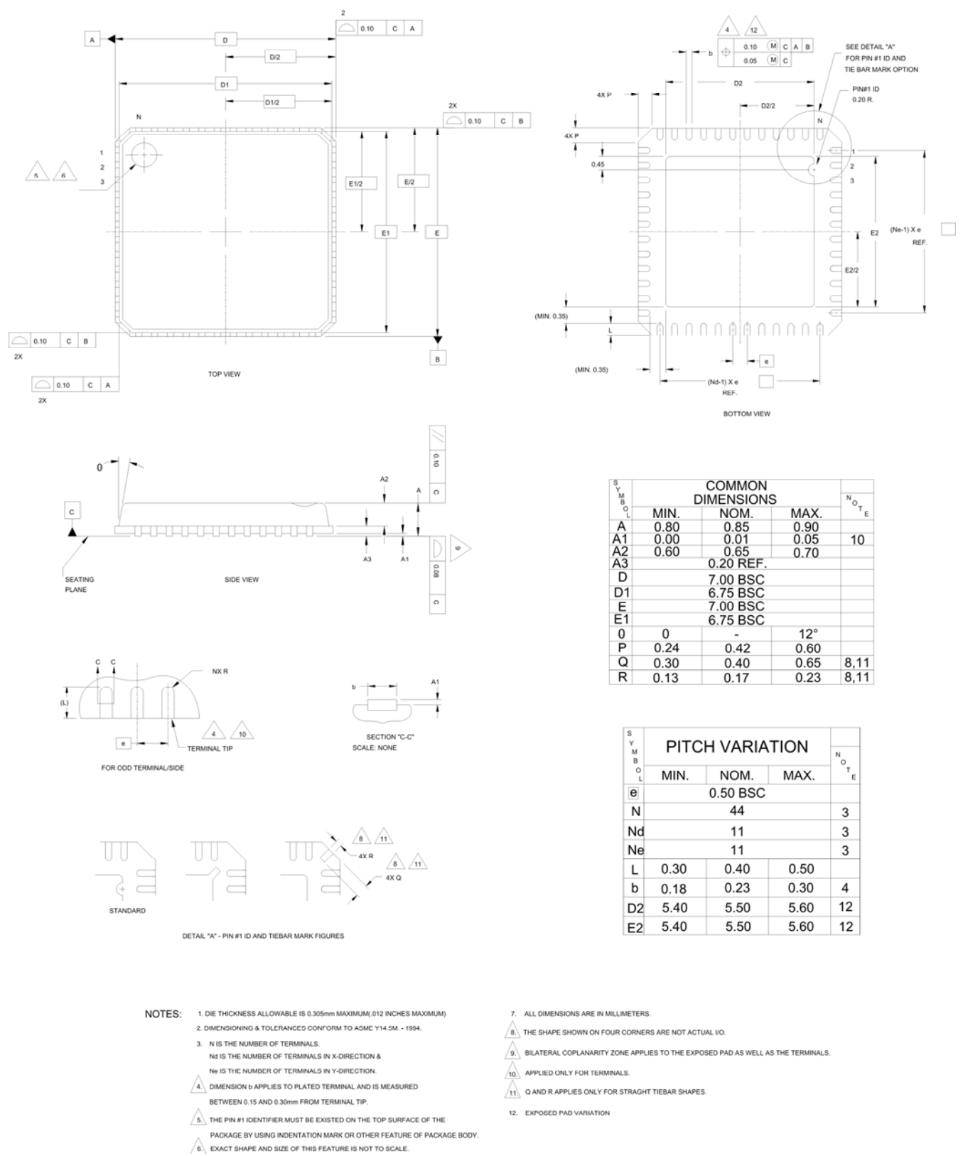
Figure 3: AMIS-49250 Package Dimensions (44-pin NQFP)
