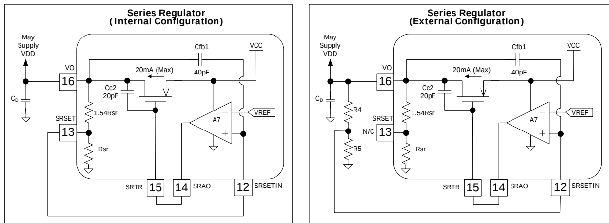
Figure 5: Series Regulator
