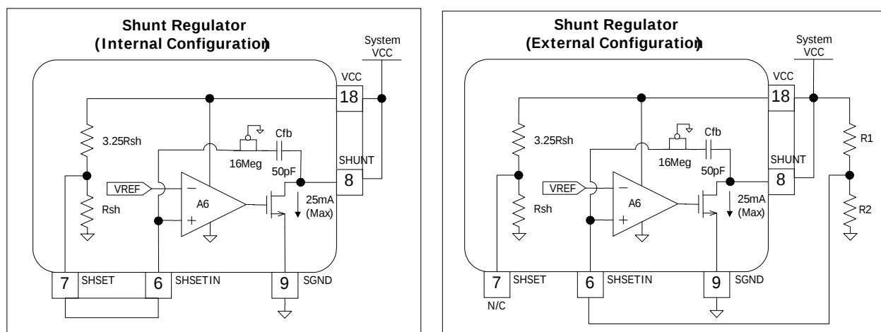
Figure 4: Shunt Regulator
