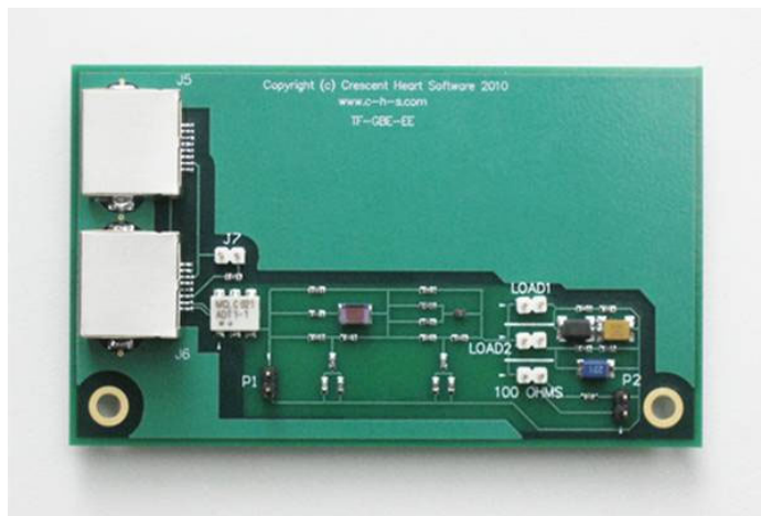
TF-GBE-EE Test Fixture for Energy Efficient Ethernet measurements on 10BASE-Te.
