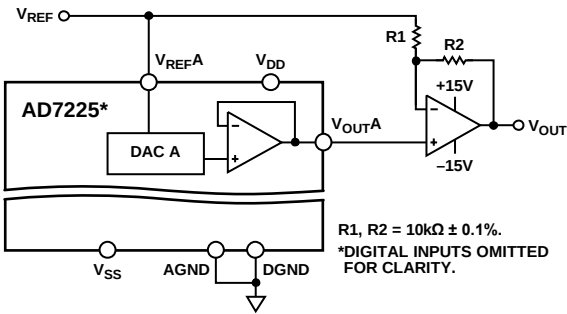
Figure 17. Bipolar Output Circuit
