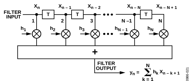
Figure 21. Transversal Filter
