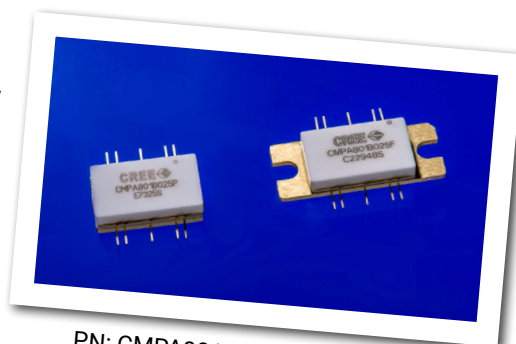
PN: CMPA801B025F/ CMPA801B025P Package Type: 440208 / 440216
