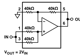
Figure 46. Noninverting Amplifier, Gain = 2
