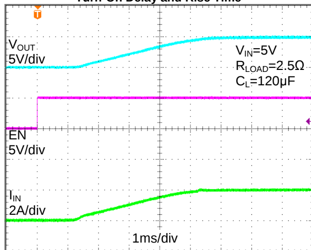
Turn-On Delay and Rise Time
